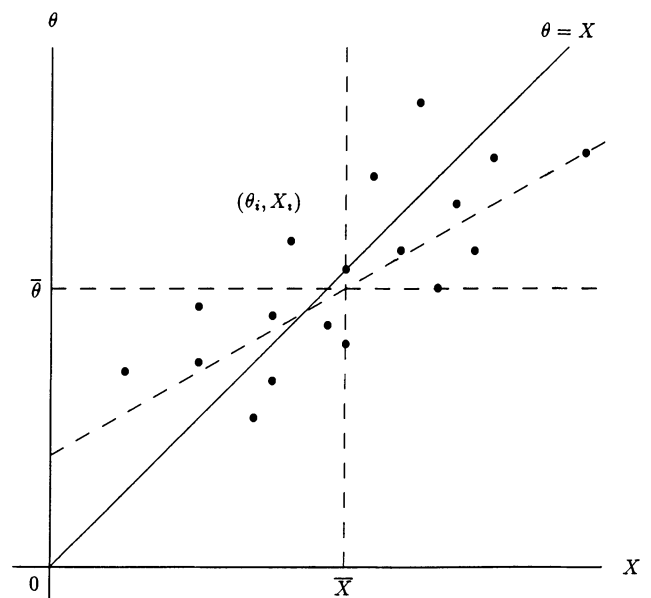
FIG. 1. Hypothetical bivariate plot of \theta_i vs. X_i , for i = 1, \dots, k .
